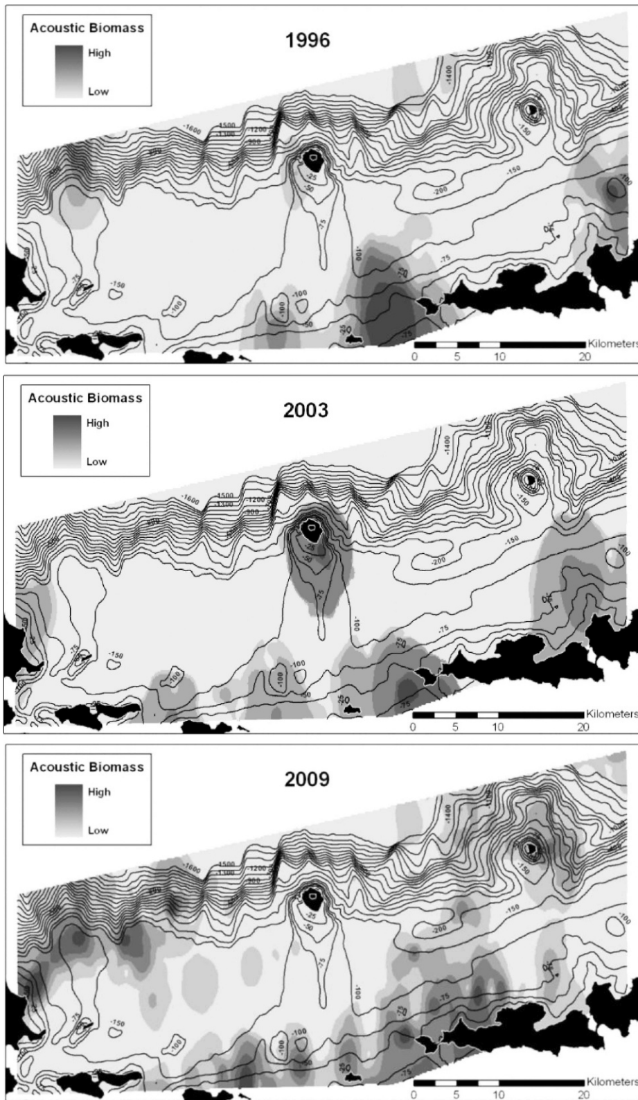
FIGURE 5. Distribution of acoustic biomass for the top 50 m of the water column for the Kasatochi study area. Maps are based on IDW interpolation of relative acoustic biomass. Relative measurements are presented owing to use of different hydro-acoustic systems or instrument settings in each year.
