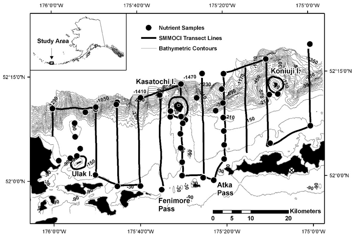
FIGURE 1. Location of the Kasatochi study area in the central Aleutian Islands with place names, sampling stations, and transects in the study area. Bathymetric contours illustrate the position of Kasatochi atop the Aleutian Ridge. Data were collected in 1996, 2003, and 2009.
