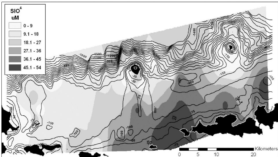
FIGURE 3. Distribution of major nutrients in the Kastochi study area July 2009. Bathymetric contours (m) are displayed for reference. Samples were taken at 10 m depth. See Figure 1 for station locations.
