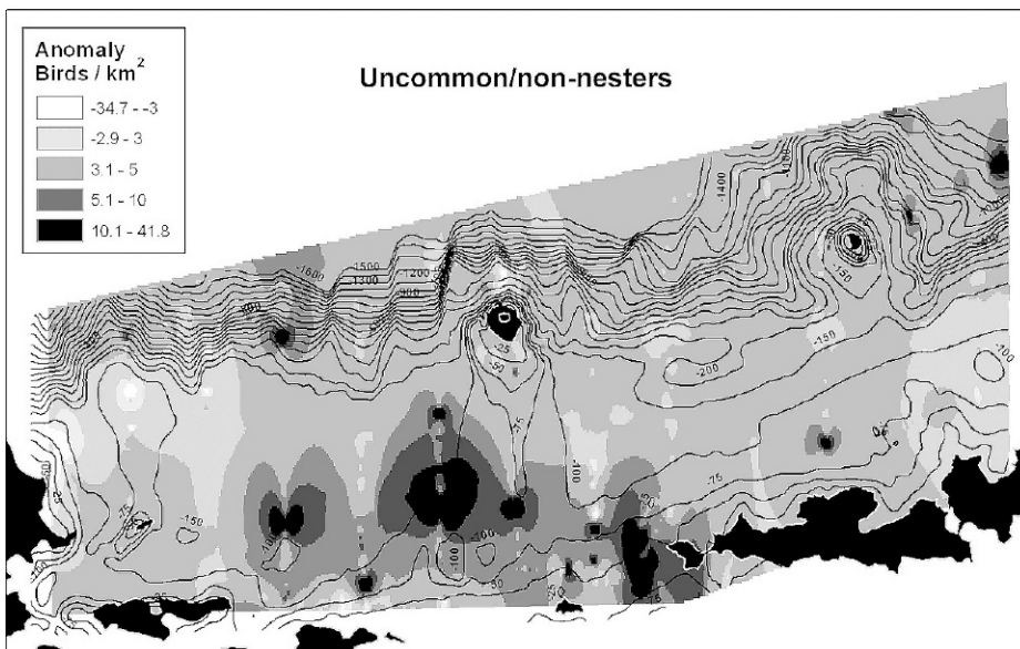
FIGURE 7. Anomaly maps (pre-eruption minus post-eruption) of seabird distributions in the study area. Light colors indicate areas of higher densities following post-eruption, dark colors indicate areas that had lower densities following the 2008 eruption.
