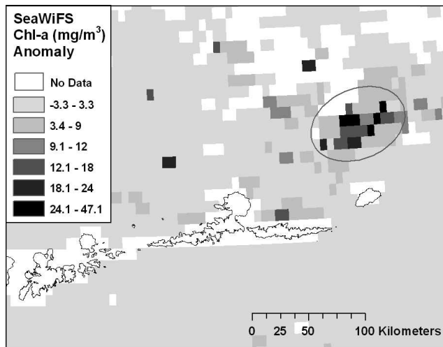
FIGURE 4. Anomaly map (post-eruption minus pre-eruption) of chlorophyll- a concentrations following the 7–8 August 2008 eruption. Pre-eruption layer was the mean of September 2003–2007. Dark colors indicate areas of anomalously high chlorophyll- a concentration estimated with SeaWiFS imagery. The ellipse designates a contiguous area of anomalously high chlorophyll- a .
