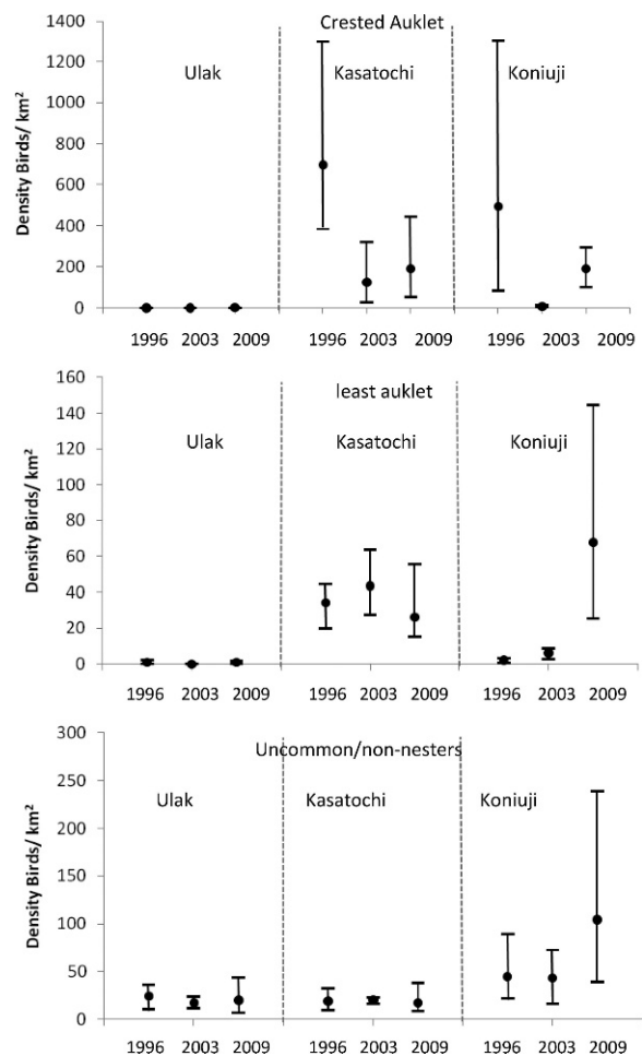
FIGURE 6. Densities for least auklet, crested auklet and uncommon/non-nesters for the three colony islands within the study area (Ulak, Kasatochi and Koniuji) for the three sampled years (1996, 2003, and 2009). Error bars represent 90% CIs of densities.
