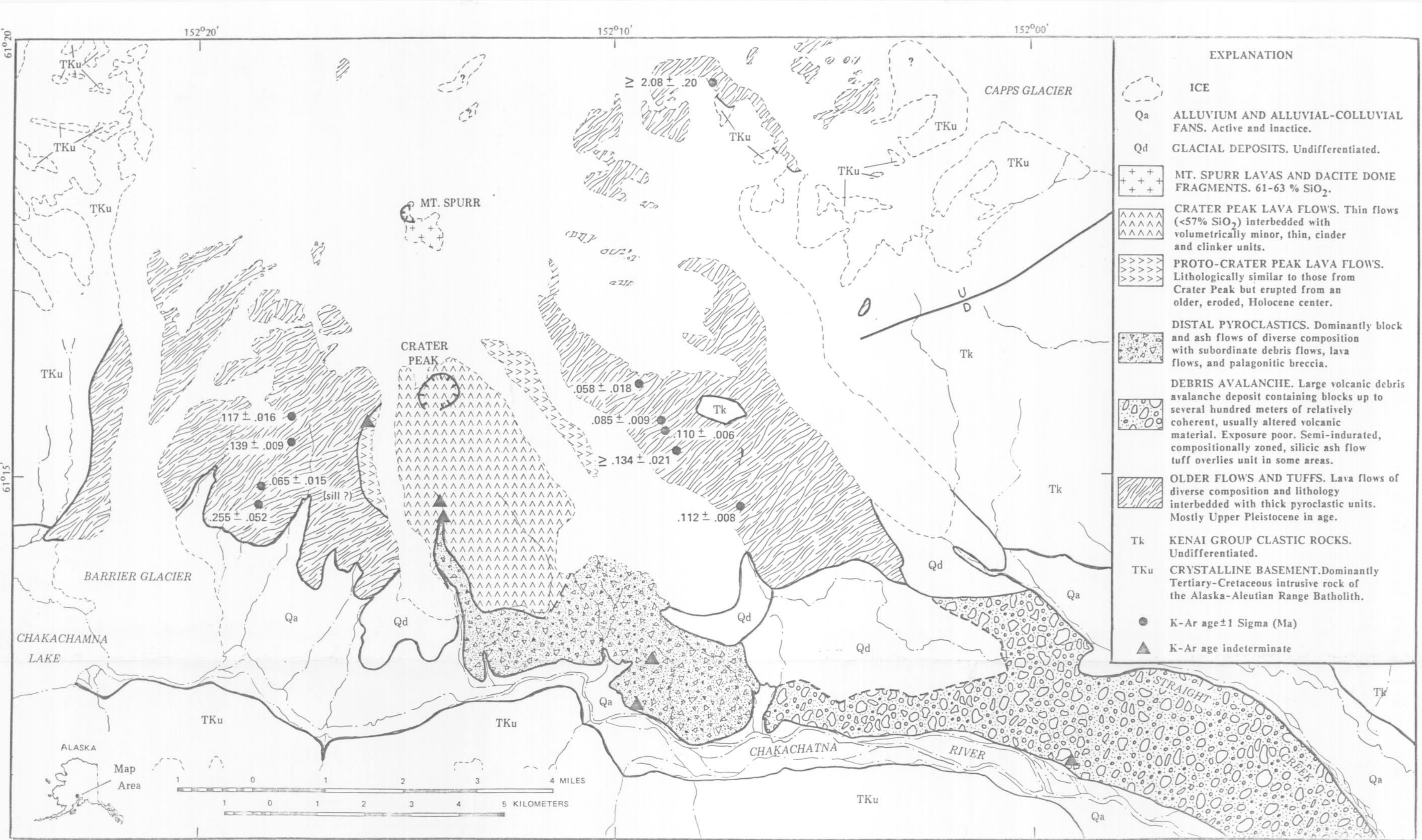
Plate 1-1: Mt. Spurr, Alaska, Reconnaissance geologic map and K-Ar ages
