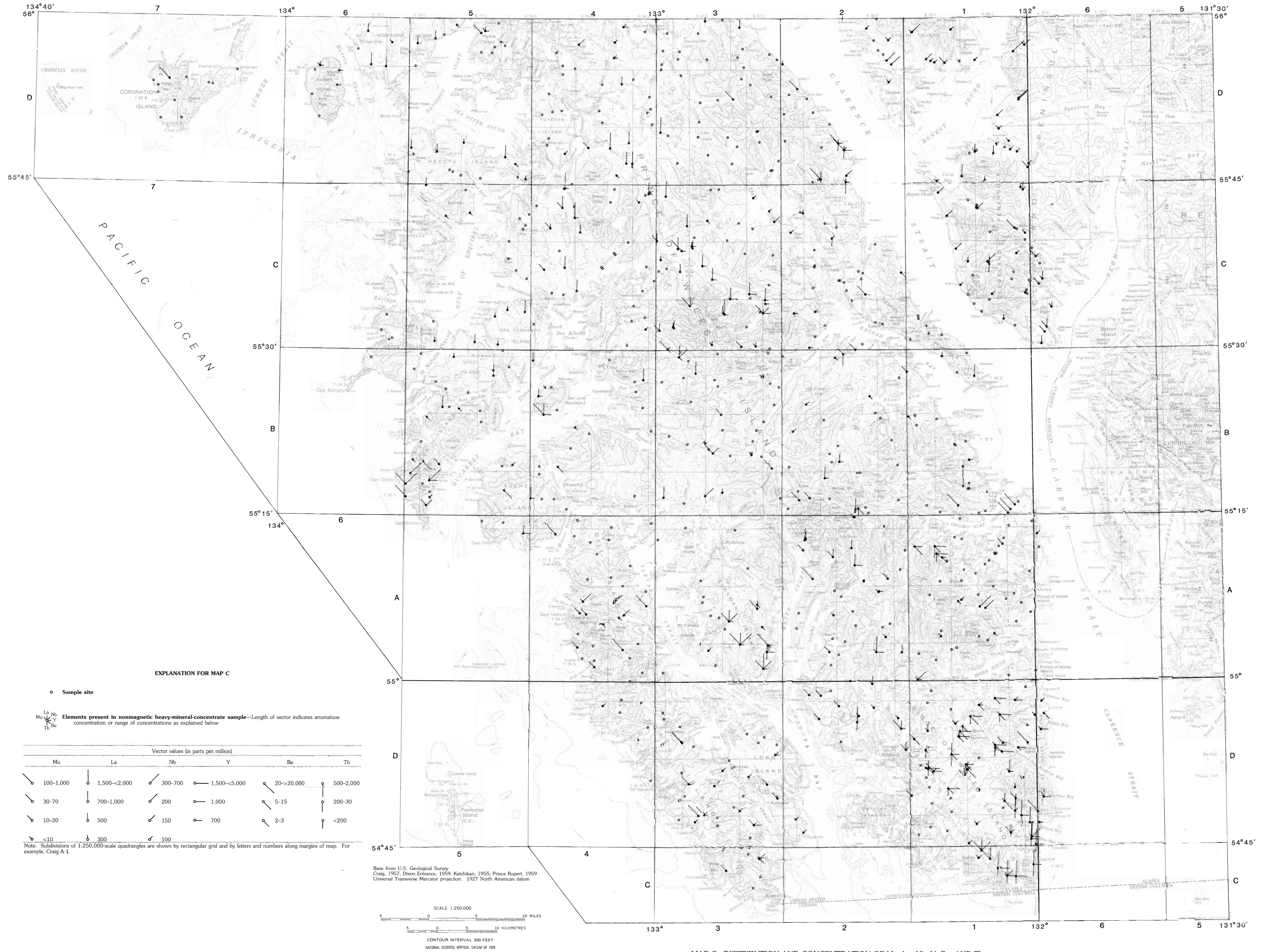
MAP C. DISTRIBUTION AND CONCENTRATION OF Mo, La, Nb, Y, Be, AND Th
