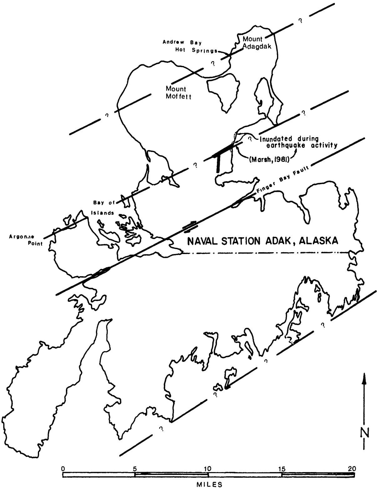
FIGURE 23. Map of Adak Island Indicating Possible en Echelon Faulting on a Strike of N60°E.
