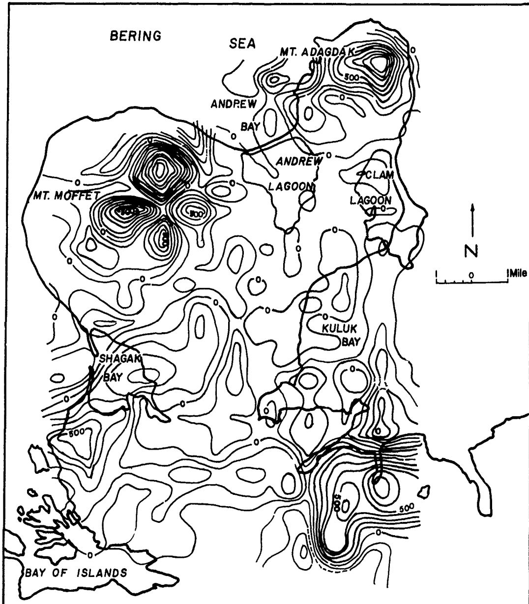
FIGURE 6. Second Vertical Derivative Map of Northern Adak Island. Contour interval 100 \gamma mas/(0.5 mile) (from Keller et al, 1954).
