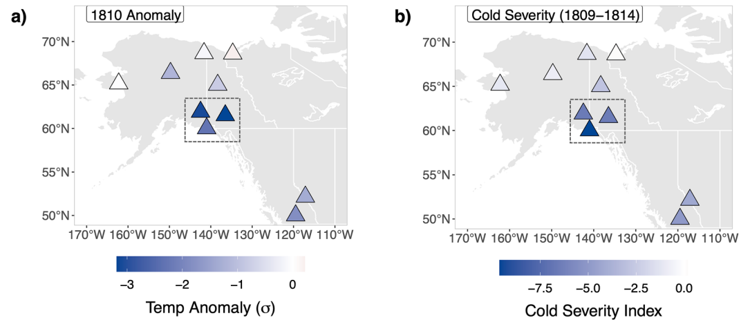
Figure 3. The spatial signature of cold temperatures across NWN after the 1809 eruption. For each record, we show the 1810 temperature anomaly, expressed as z -scores relative to 1680–1990 (a) and the cold severity index (b), calculated as the magnitude of cooling multiplied by the number of years with a below average temperature from 1809 to 1814. The dashed box represents the three records (GOA, WRA, YUK) with the most pronounced cooling signature after the 1809 eruption.
