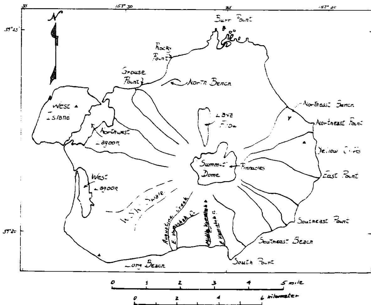
Figure 2. Augustine Island. Most place names are informal but are needed in present report for locations and designation of geologic map units. Mostly informal place names proceed north from summit then clockwise around coast. SD, summit-dome complex; NSL North Slope lava flow; BP, Burr Point; NEB, Northeast Bench; NEP, Northeast Point; YC, Yellow Cliffs; EP, East Point; SEP, Southeast Point; SEB, Southeast Beach; SP, South Point; KD, Kamishak Dome; LB, Long Beach; WL, West Lagoon; WI, West Island; NWL, Northwest Lagoon; GP, Grouse Point; NB, North Bench; RP, Rocky Point.
