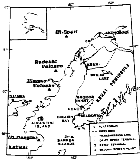
Figure 1. Index map of Cook Inlet, Alaska. Augustine volcano constitutes most of Augustine Island.
