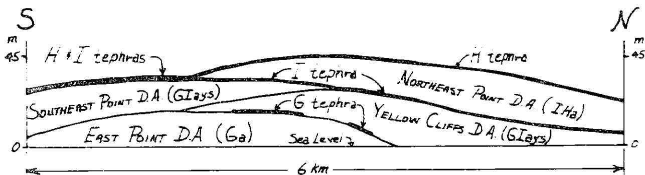
Figure 7. Schematic sketch of coastal cliffs along east side of Augustine Island showing stratigraphic relations of four oldest debris-avalanche deposits and the three oldest of the coarse pumiceous-tephra "marker beds"
