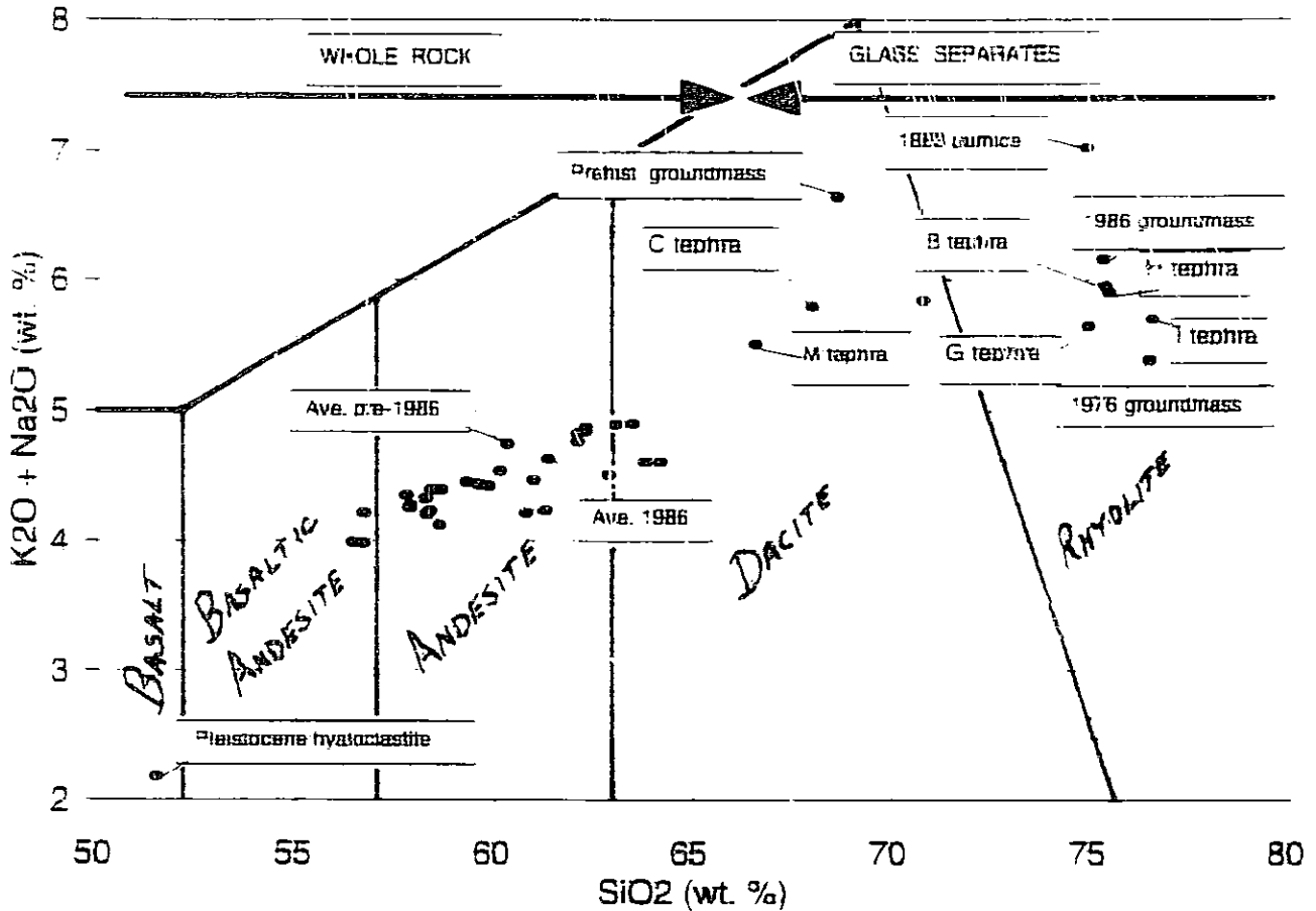
Figure 4. Plot of chemical analyses of rocks (whole-rock analyses) and tephra (glass separates) from Augustine Island. Graphed data compiled from Kienle and Forbes (1976), Daley (1986), Swanson and Kienle (1988), Siebert and others (1989), and from selected analyses by James R. Riehle in 1995 of tephra samples collected during present project. Boundaries of named fields according to LeBas and others (1986) and LeBas and Streckensen (1991, fig. 5).
