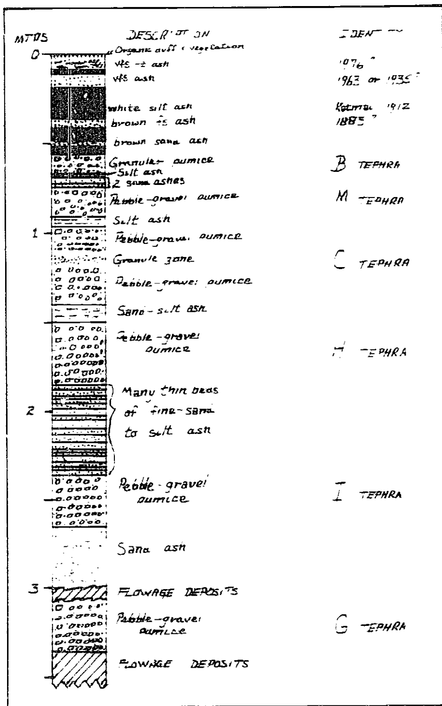
Figure 5. Tephras stratigraphy overlying flowage deposits just north of Southeast gully about 0.9 km coastwise north-northeast from Southeast Point. The "flowage deposits" are each several meters thick. fs = fine sand; vfs = very fine sand; z = silt.
