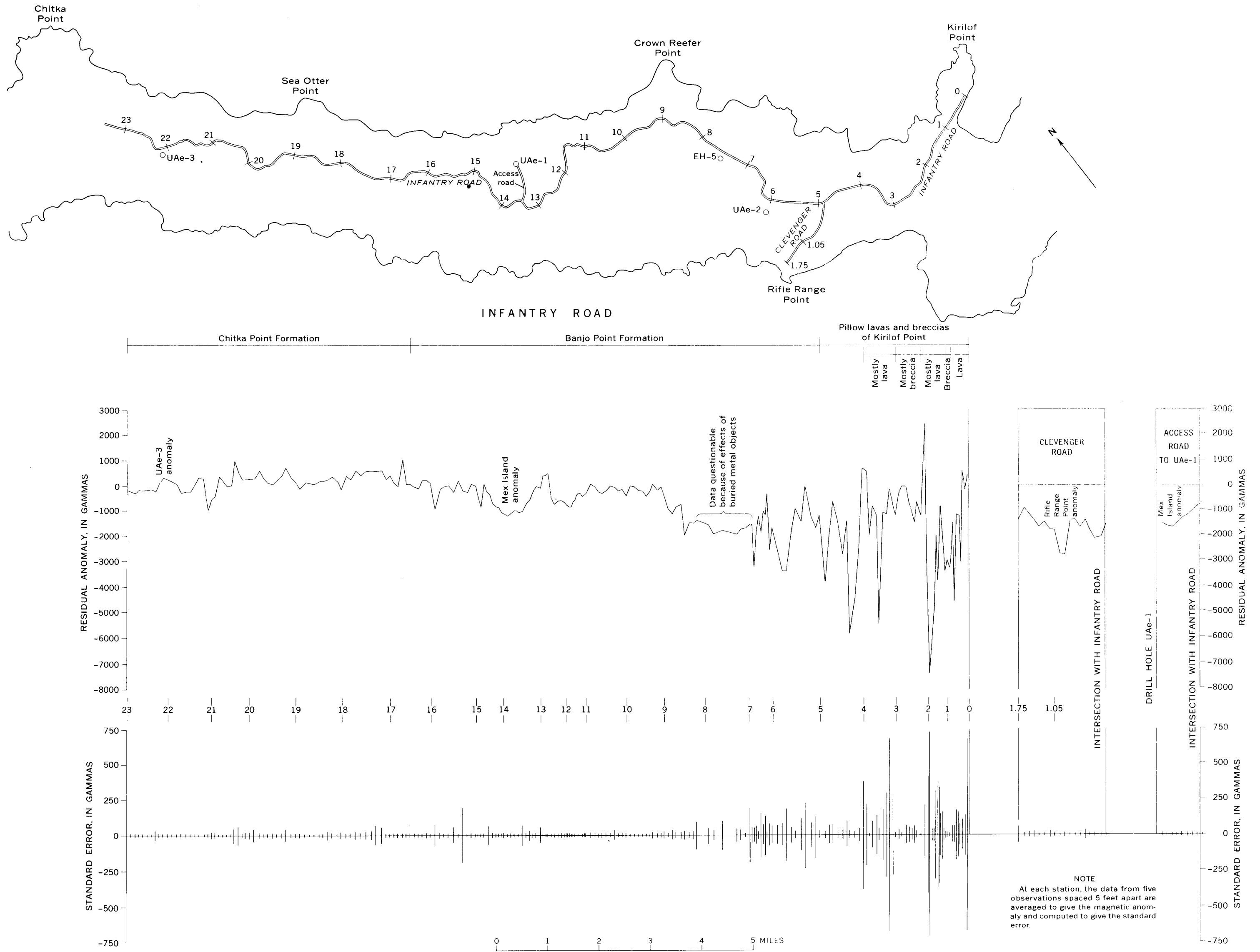
PLOTS OF MAGNETIC ANOMALY AND STANDARD ERROR FROM GROUND SURVEY DATA AT STATIONS 0.1 MILE APART ON AMCHITKA ISLAND, ALASKA
