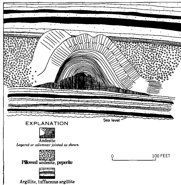
FIGURE 14.—Derby-shaped layered lava pod exposed in three successive small headlands along coast east of Tower Point, Unalaska Island; drawn from a series of photographs. Dissection is sufficient to indicate that a cross section taken perpendicular to the coast would be identical. Central derby is younger than coarsely columnar carapace which grades laterally into pillowed lava.
