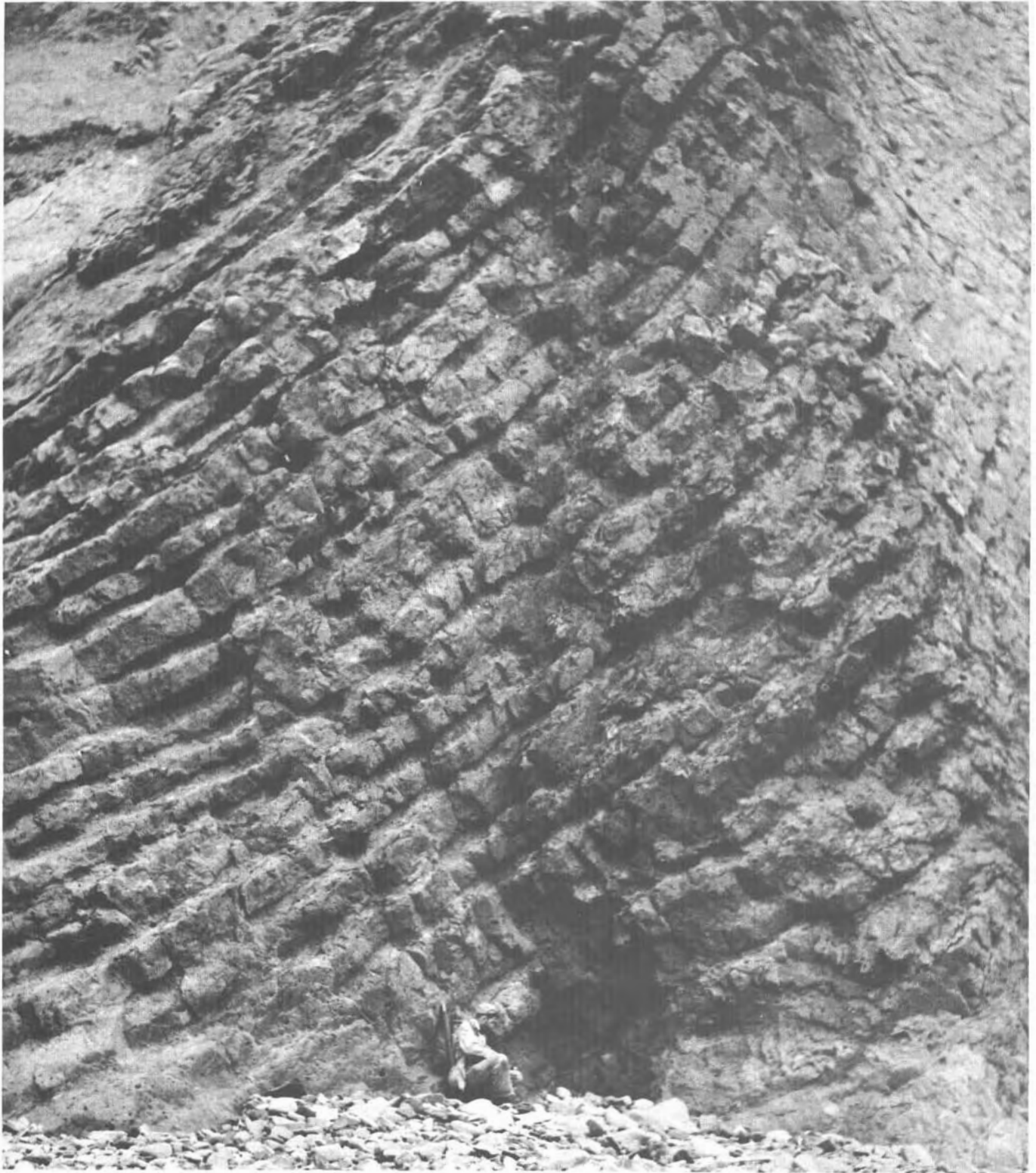
FIGURE 9.—Layered albitized dacite in active sea cliff on east side of Buttress Point, Unalaska Island. Upper contact of lava pod against small lens of tuffaceous sediment shown in upper left of photograph; for detail see figure 10. Photographed from the same place as figure 8 but from the opposite direction.
