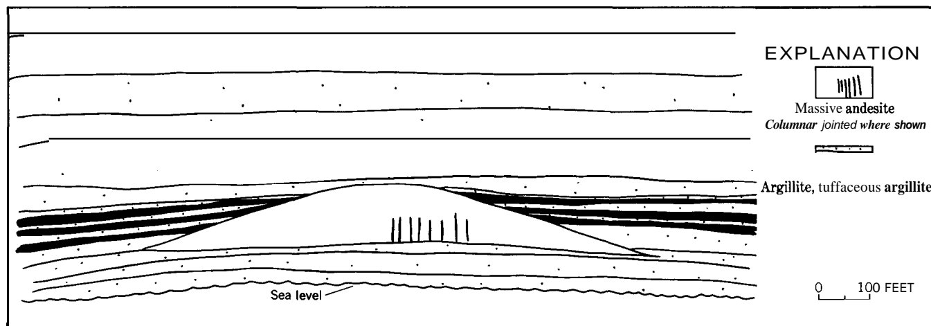
FIGURE 3.—Section of laeolith intruding rocks exposed in sea cliff south-southeast of Spray Cape, Unalaska. Drawn from a photograph.
