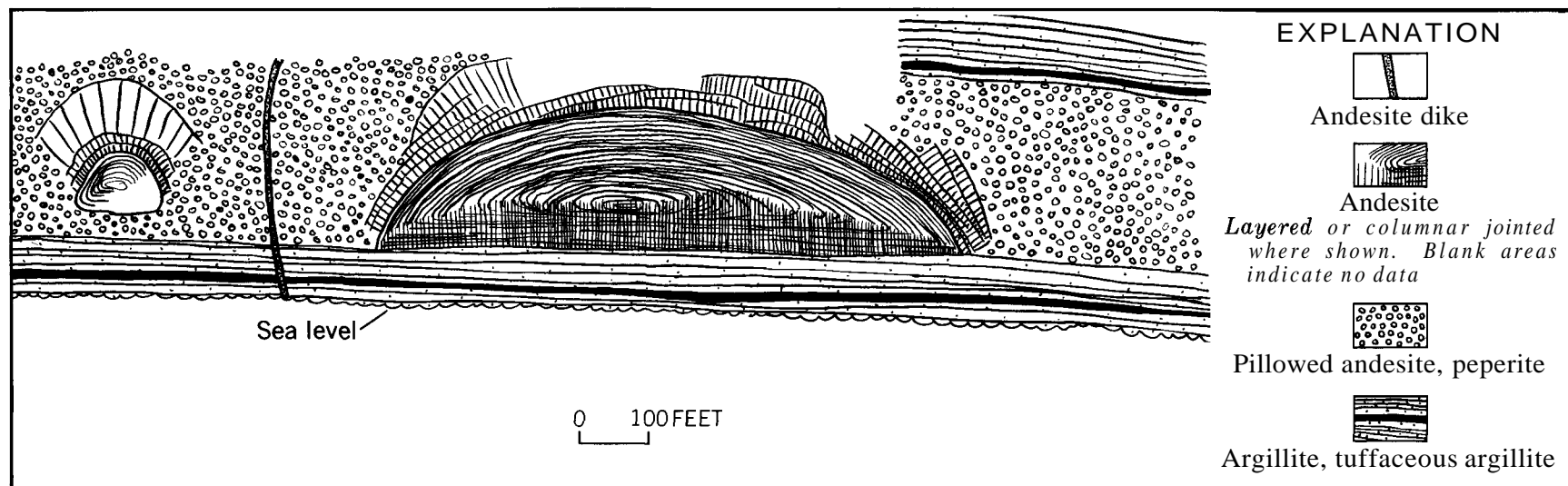
FIGURE 15.—Restored section of semiellipsoidal layered lava pod exposed on three successive small headlands midway between Tower Point and Lion Bight, Unalaska Island; drawn from a photograph. Dissection is sufficiently complete to indicate that a cross section taken perpendicular to the coast would be identical. Central ellipsoid is younger than coarsely columnar carapace which grades laterally into pillowed lava.
