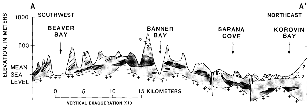
Figure 3. Schematic and interpretive cross-section of Atka Island.
