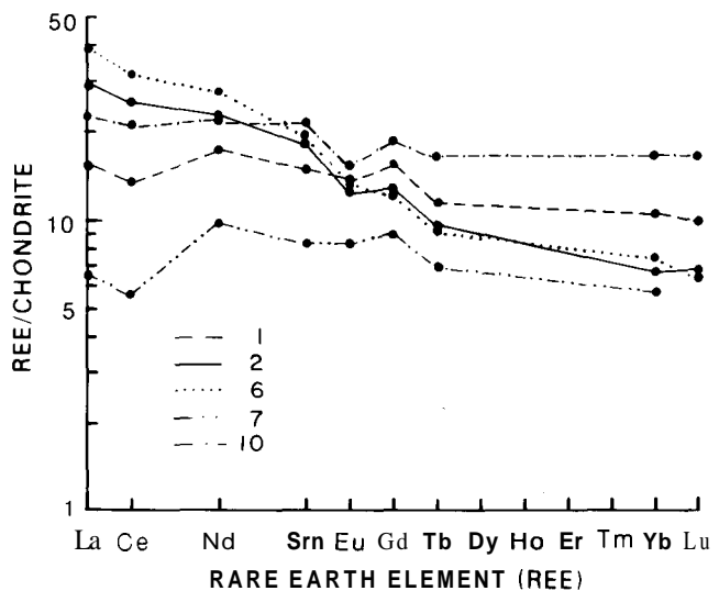
Figure 8. Rare-earth element (REE) plot for selected rocks from Atka Island (tables 6, 7). Sample 7 is extremely depleted in REE, and sample 10 has a small Eu anomaly.
