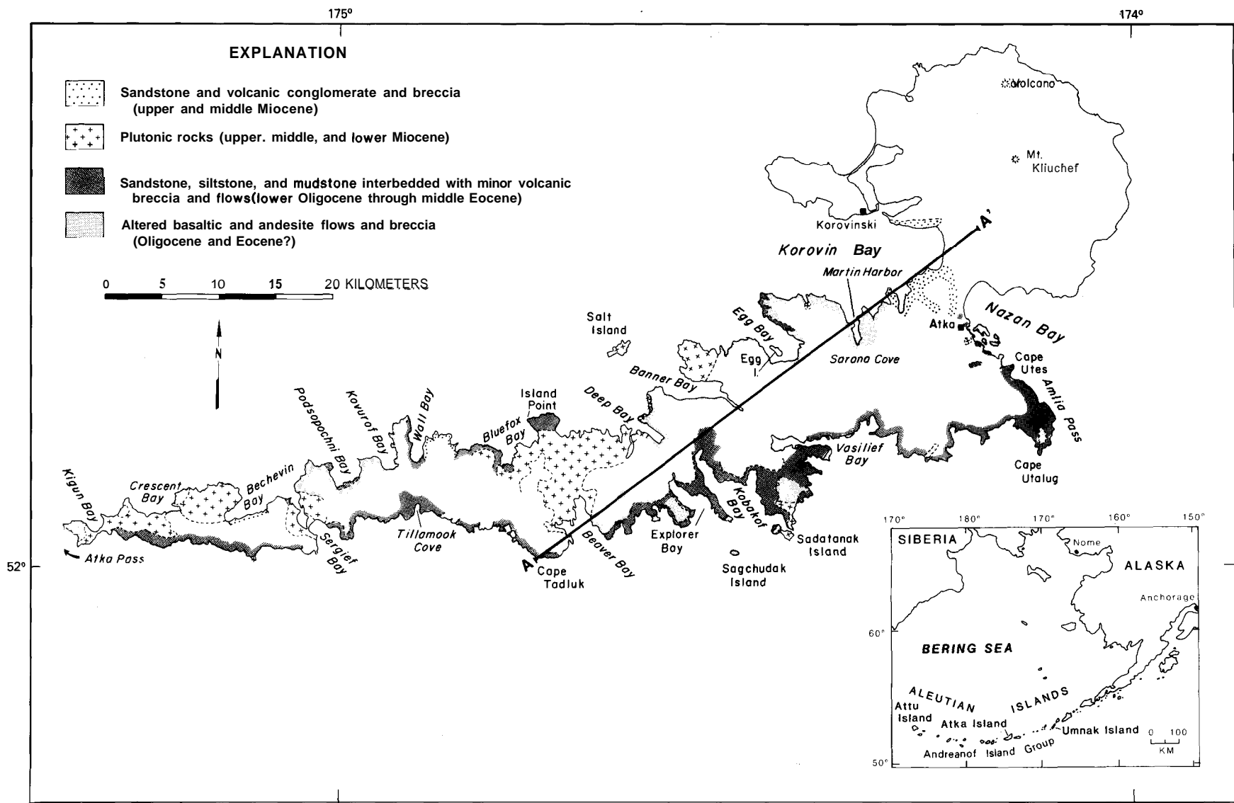
Figure 1. Geologic map of Atka Island, showing location of cross section A-A' in figure 3.
