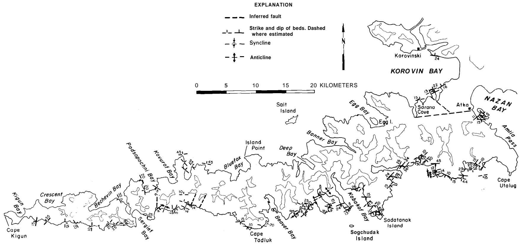
Figure 2. Structural map of Atka Island. Irregular outlines are 1000-ft contour.
