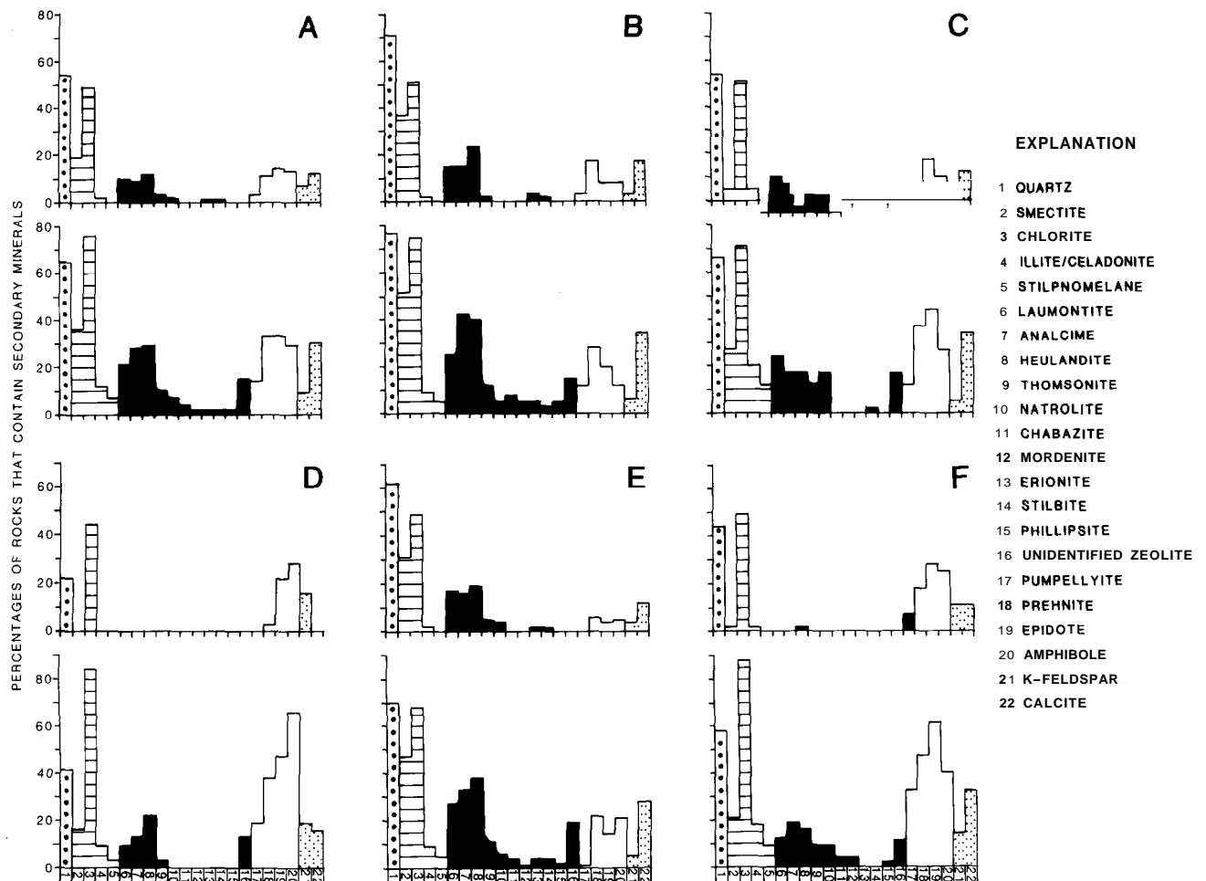
Figure 9. Alteration products of Atka Island rocks. A , All rocks, based on 138 samples. B , Sedimentary rocks, based on 65 samples. C , Volcanic and pyroclastic rocks, based on 41 samples. D , Plutonic rocks, based on 32 samples. E , All rocks from east half of island, based on 81 samples. F , All rocks from west half of island, based on 57 samples. Upper histograms are for only extensively altered rocks; lower histograms are for all altered rocks within each numbered category.
