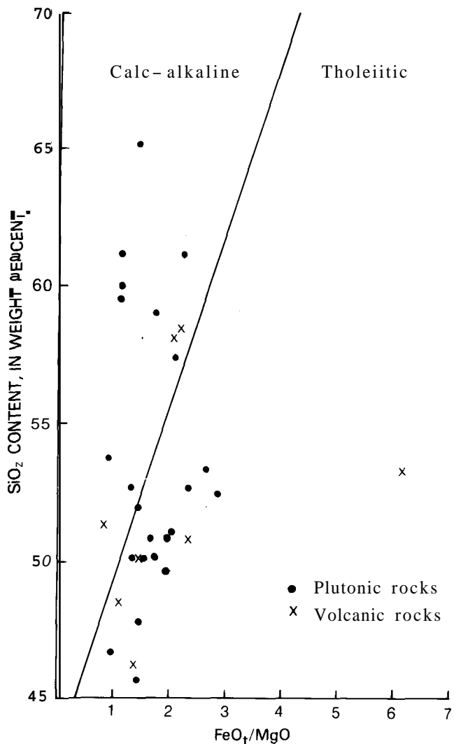
Figure 6. \text{SiO}_2 content versus \text{FeO}_T/\text{MgO} ratio for Tertiary rocks of Atka Island after (Miyashiro, 1974, and R. Kay, 1977). Analytical data from L. A. Morgenson and others (unpub. data, 1983). Values not corrected for \text{H}_2\text{O} and \text{CO}_2 contents.
