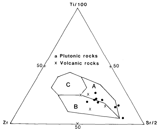
Figure 7. Triangular diagram of Sr-Ti-Zr content of plutonic and volcanic rocks (after Pearce and Cann, 1973). All mafic rocks from Atka Island plot in or near the A (low potassium tholeiite) and B (calcalkaline basalt) fields.
