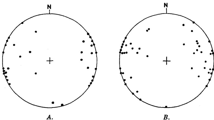
FIGURE 2. —Stereographic plot of (A) 36 poles to strain-slip cleavage in shoreline exposures from Rodman Bay to Hanns Bay and (B) 51 poles to strain-slip cleavage in Kelp Bay. Data are projected to lower hemisphere.
