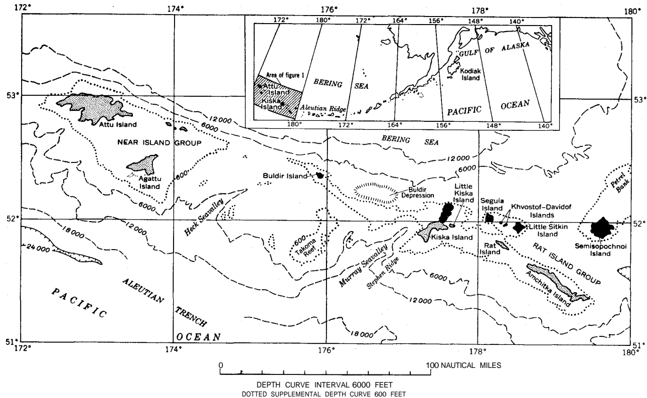
FIGURE 80.—Location of the Aleutian Islands and Kiska Island on the western Aleutian Ridge. Stippled pattern shows islands on the southern linear element of the ridge; solid pattern shows active and dormant volcanoes on the northern linear element.
