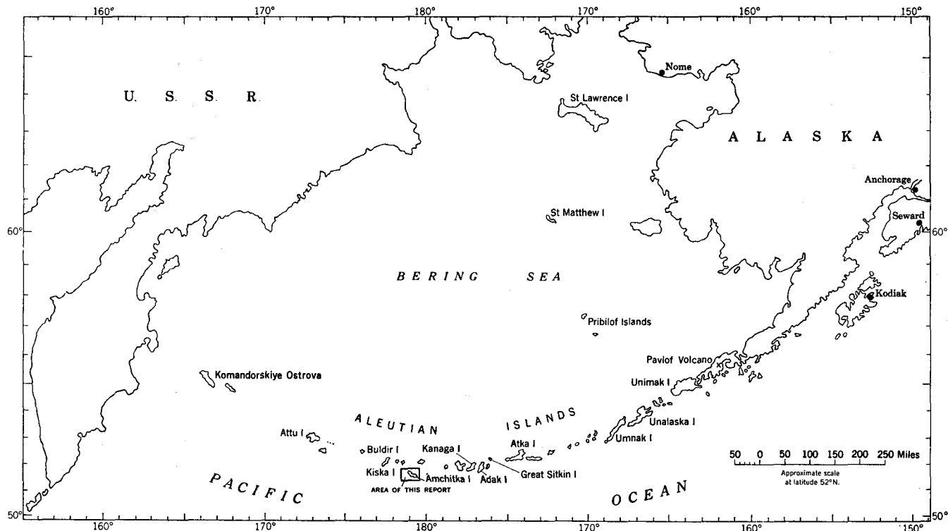
FIGURE 77.—Map of the Alaska Peninsula and Aleutian Islands.
