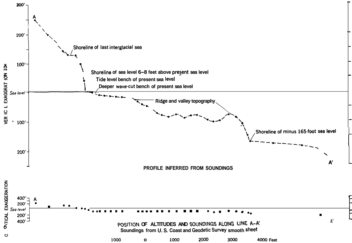
FIGURE 78.—Profile of Chitka Point and offshore area, with inferred origin of features. (See pl. 69 for location of profile.)
