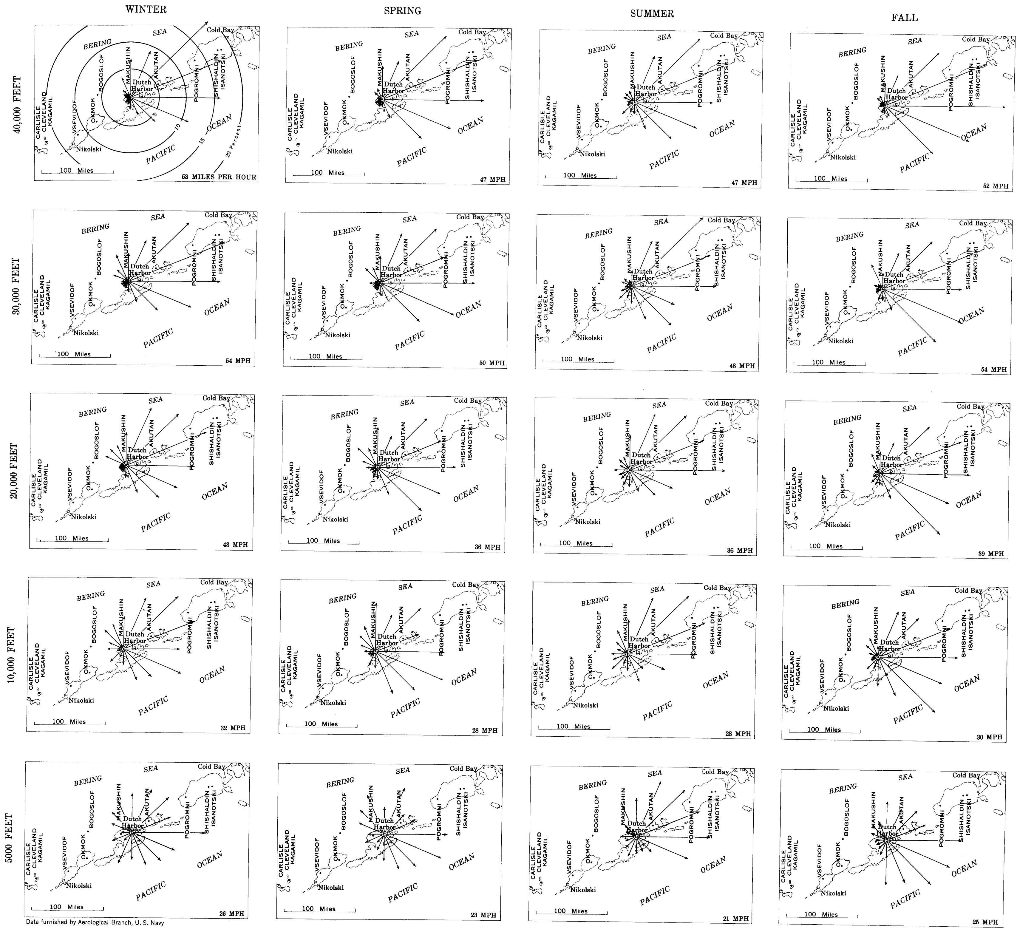
MAP MONTAGE OF AVERAGE UPPER-AIR WIND DIRECTIONS FOR DUTCH HARBOR, ALASKA, 1948-53 WITH WIND ROSES FOR HIGHER LEVELS CENTERED ON MAKUSHIN VOLCANO Arrows fly with the wind and lengths represent percentages of time. Average wind speed in miles per hour is noted in lower right corner of each map
