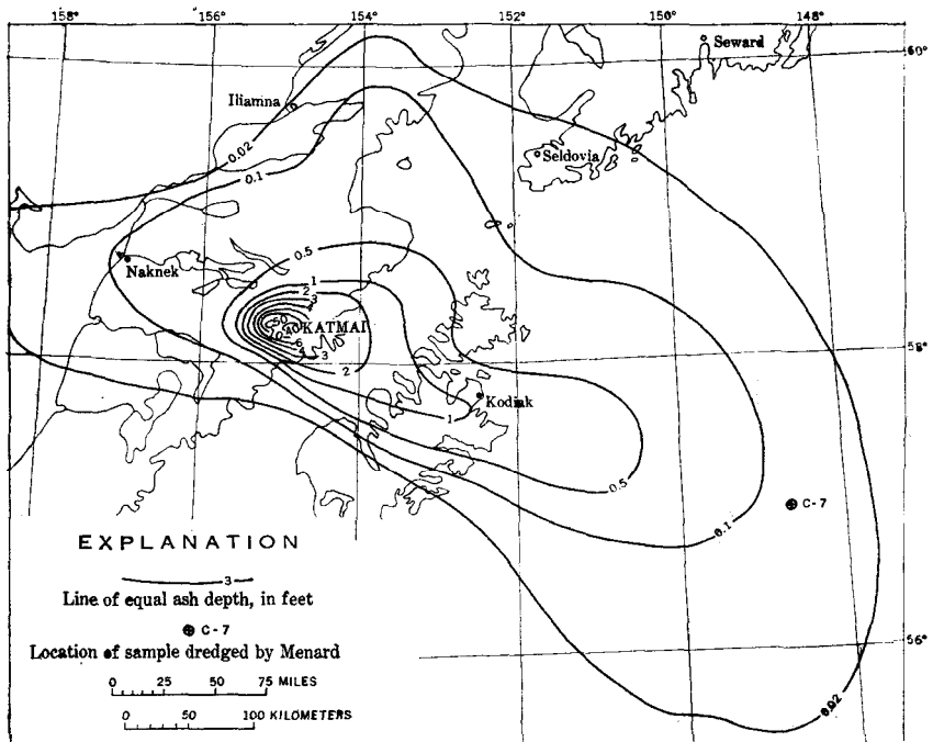
FIGURE 62.—Map of Mount Katmai and the Valley of Ten Thousand Smokes, Alaska showing thickness of ash deposit from the eruption in June 1912 (after Griggs, 1922, and Menard, 1953).
