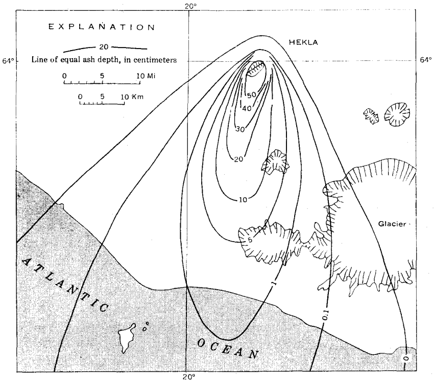
FIGURE 64.—Map of Hekla volcano in Iceland showing thickness of ash deposit from the eruption in March 1947 (after Thorarinsson, 1964).
