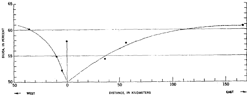
Figure 70.—Graph showing variation in silica content of ash fall of Gunung Kelud in Java, in 1919, with distance east and west of the volcano (from data listed by Mohr and Van Baren, 1964, p. 233).
