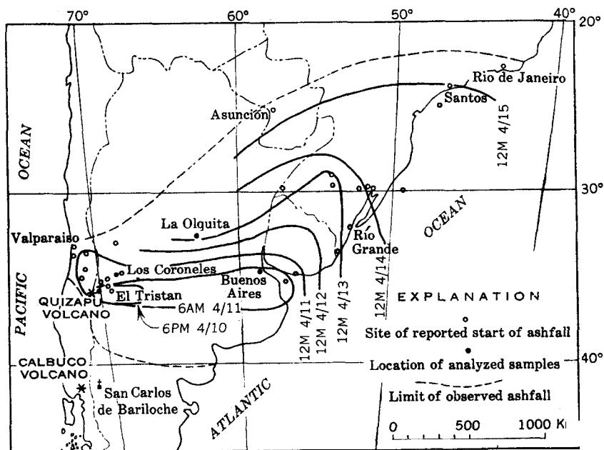
FIGURE 67.—Map of successive positions of ash front from the eruption of Volcán Quizapú in Chile, in April 1932 (after Larsson, 1937).
