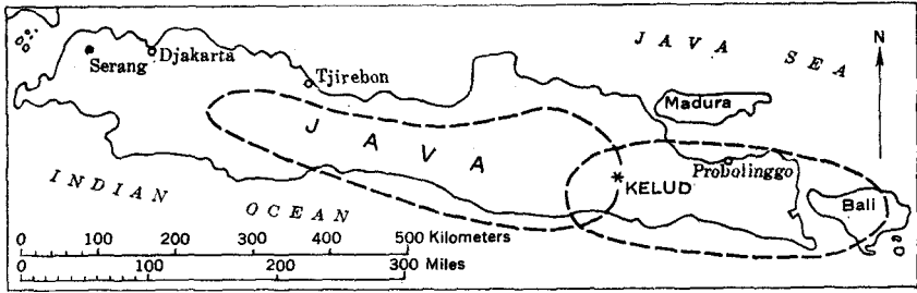
Figure 69.—Map of Java, showing bilateral distribution of ash fall from the 1919 eruption of Gunung Kelud volcano. Dashed lines enclose areas of ashfall. (Mohr and Van Baren, 1964, fig. 38a, after Kemmerling, 1921).
