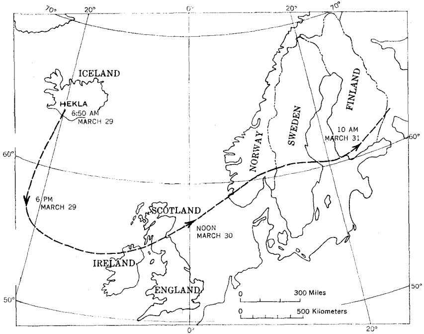
FIGURE 66.—Map of route of airborne ash from the eruption of Hekla volcano in Iceland, across Scotland and Finland, on March 29–31, 1947 (after Thorarinsson, 1964).
