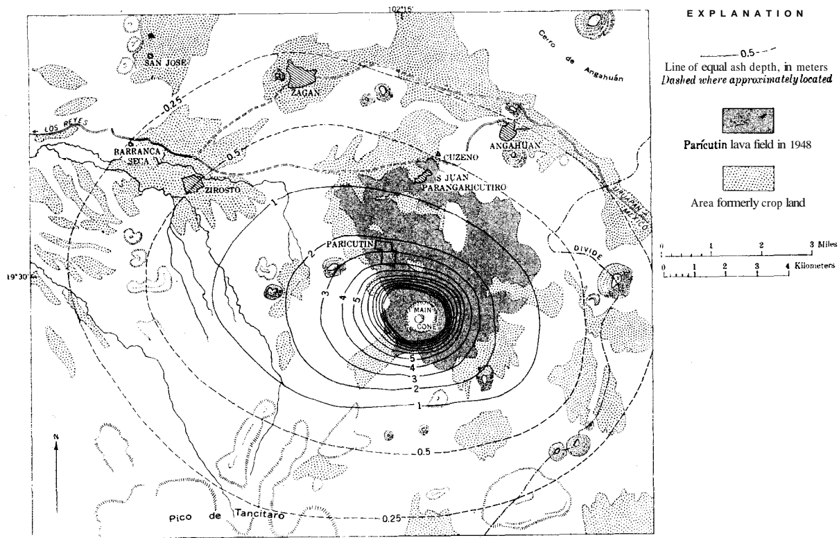
FIGURE 71.—Map of the vicinity of Parícutin in Mexico (from Segerstrom, 1950, pl. 8), showing thickness of ash deposit in 1946 from the eruption of the volcano, the area covered by lava flows in 1948, and the area that was crop land before the beginning of the eruption in 1943.
