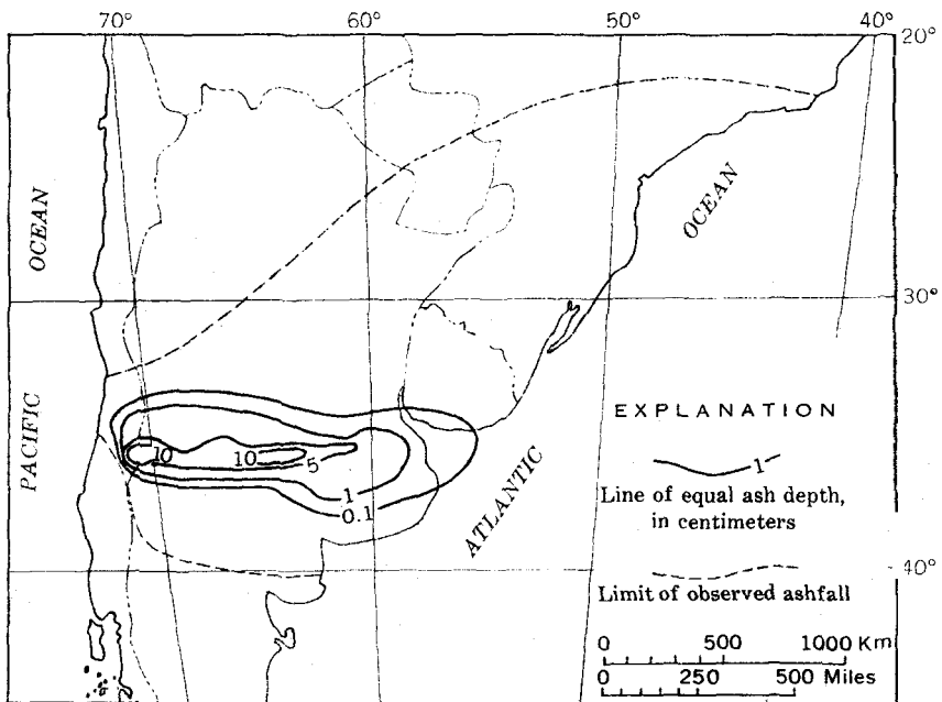
FIGURE 68.—Map showing the thickness of ash deposits from the eruption of Volcán Quizapú, Chile. In April 1932 (after Larsson, 1937).
