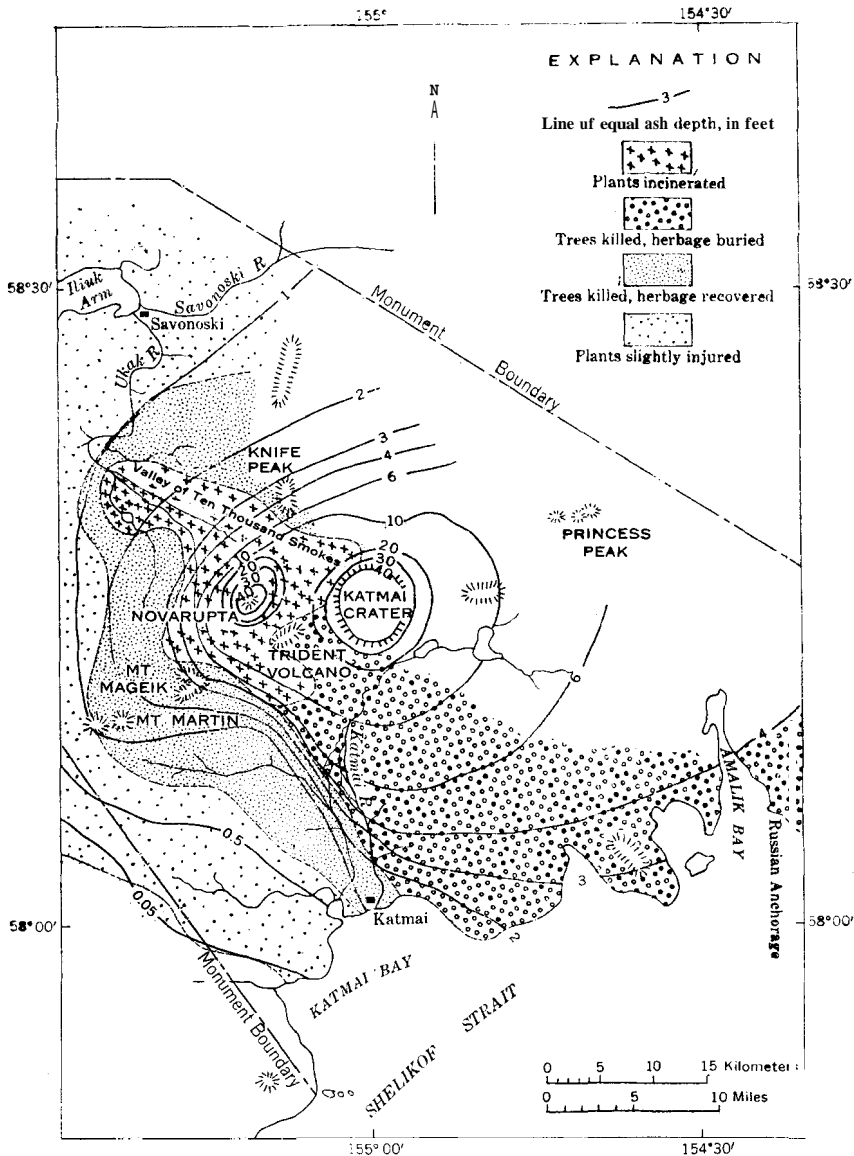
FIGURE 72.—Map of Mount Katmai, Alaska, showing destruction of vegetation in 1912 by the eruption and thickness of ash deposit (after Griggs, 1919b).
