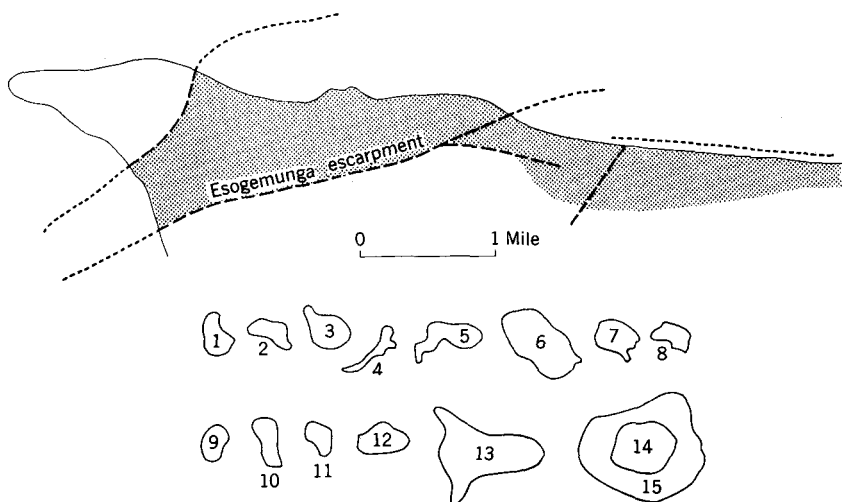
FIGURE 34.—The tuff conduit at Esogemunga, St. George Island (diagonally hatched) compared with tuff necks from Kimberley, South Africa (1–8) and from Schwaben, Germany (9–15). 1, Bulfontein; 2, Weselton; 3, Kaffyfontein; 4, Ottos-Kopje; 5, Du Toitspan; 6, Premier; 7, Jagersfontein; 8, De Beers; 9, Grafenberg; 10, Florian; 11, Metzinger-Weinberg; 12, Neuhauser; 13, Jusi; 14, Limburg; 15, Randecker Maar. (1–15 after H. Cloos, 1941).
