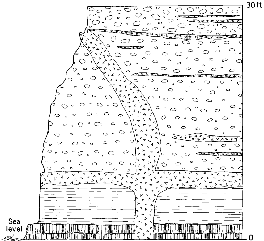
FIGURE 31.—Dike spreading out to form a sill. Section at the seashore one-third mile east of the village, St. George Island.
