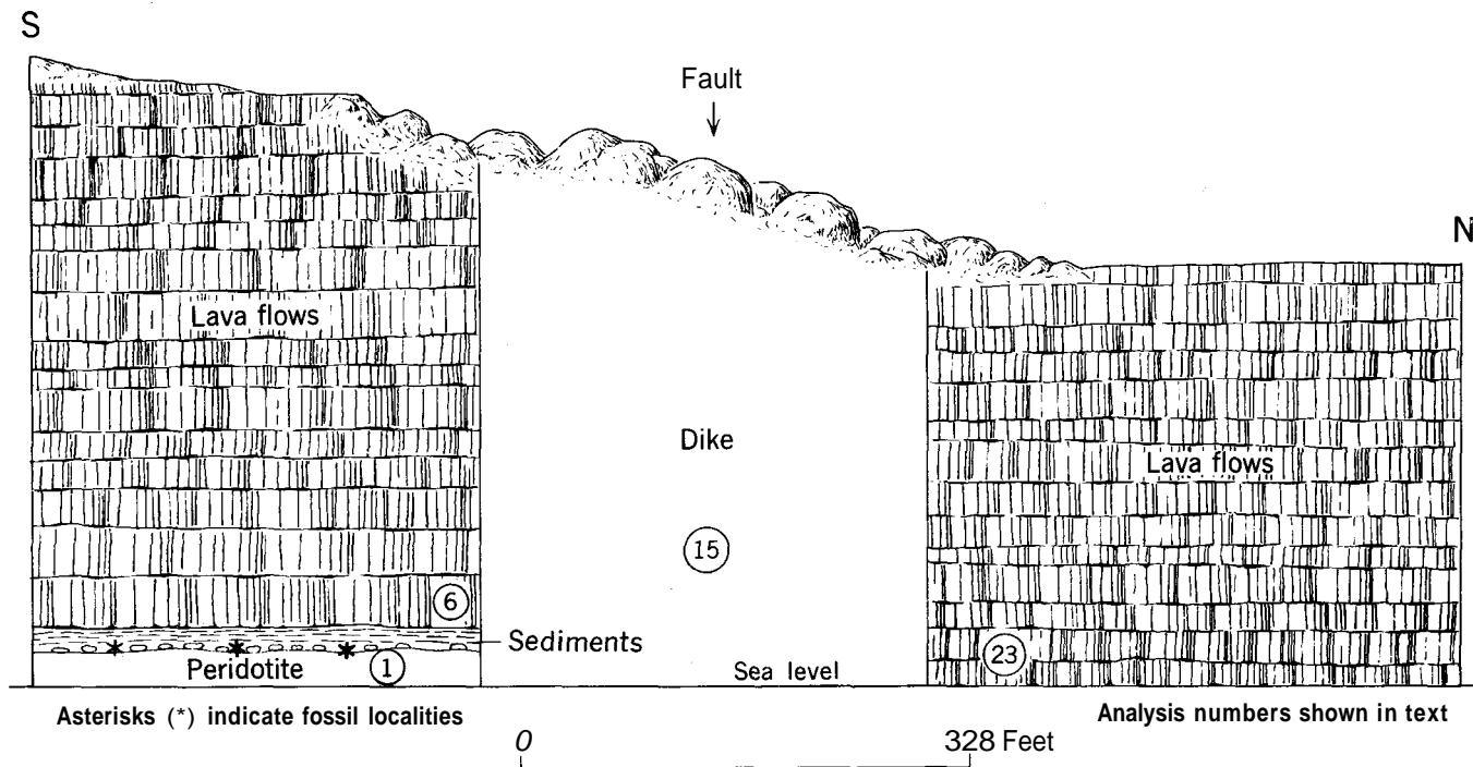
FIGURE 26.—Section about two-thirds of a mile south of Tolstoi Point, St. George Island. Numbers correspond to those of the analyzed rocks. No. 23 is described on page 115.
