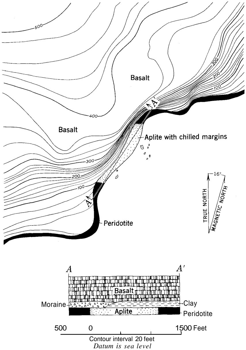
FIGURE 29.—Map of aplite intrusion, north of Garden Cove, St. George Island
