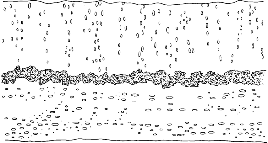
FIGURE 17.—Section one-third mile south of the village, St. Paul Island, through two flows, separated by a scoriaceous layer. In the top flow the vesicles are aligned vertically; in the bottom flow they are arranged horizontally. Total thickness, 6\frac{1}{2} feet.
