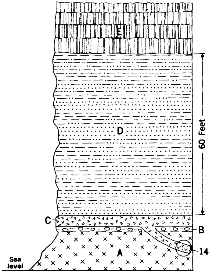
FIGURE 30.—Section at the seashore 1 mile south of Garden Cove, St. George Island. A , peridotite; B , thin layer of clay with houldrrs of peridotite; C , sill of hyalobasaltite sending an apophysis down into the peridotite; at 14 the basanite has become limburgitic (analysis 14); D , sediments, 59 feet thick, consisting of clay, sand, and tuff with fragments of peridotite; crossbedding is conspicuous; E , lava flow with incorporated sedimentary material. At the top of this lava another series of sediment is deposited and again overridden by lava flows. Total hright of the cliff is about 200 feet.
