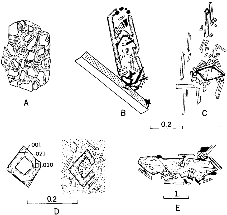
FIGURE 28.—Minerals in lavas. A, Serpentinized olivine from peridotite, Garden Cove, rock sample 1. Olivine, serpentine, and a small amount of magnetite. B, Olivine crystal in a state of resorption from plagioclase-hematite rock sample 18, top of road between village and Zapadni Bay, St. George Island. Olivine, plagioclase and hematite. C, Olivine phenocrysts and plagioclase laths illustrating preferred orientation in feldspathic basanite from rock sample 9 northeast shore of Otter Island. D, Hollow phenocrysts of olivine, plagioclase laths, and black pigments of magnetite in glass groundmass. Basanite rock sample 17 intrusive into Rush Hill, St. Paul Island. E, Resorbed olivine phenocryst in fluidal glass ground-mass). Basanite flow, Tolstoi Point, St. Paul Island. Scales in millimeters.
