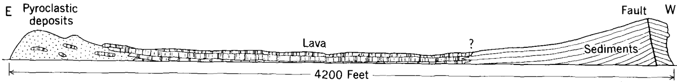
FIGURE 23.—Section of Otter Island. From east to west are pyroclastic rocks, lava, and sedimentary rocks.
