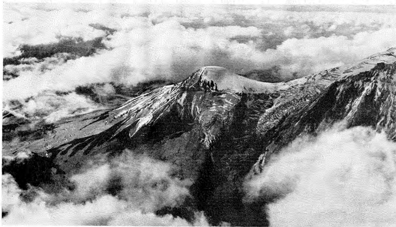
LITTLE PAVLOF VOLCANO.
