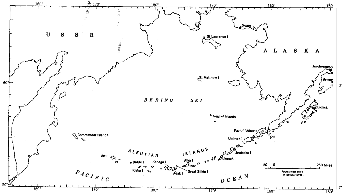
FIGURE 1.—Map of the Alaska Peninsula and Aleutian Islands.
